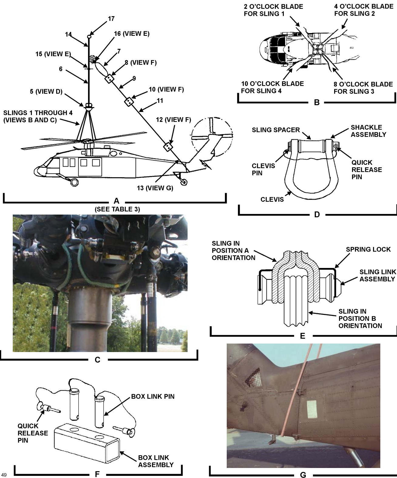
Figure 1. Disabled UH-60 and Recovery Helicopter Rigging
