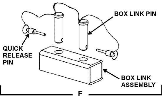
Figure 1. Disabled AH-64D and Recovery Helicopter Rigging
