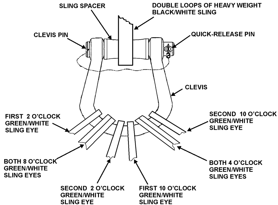
Figure 3. Rigging Shackle Assembly
